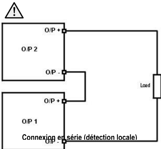
Series Wiring (Local Sense)
