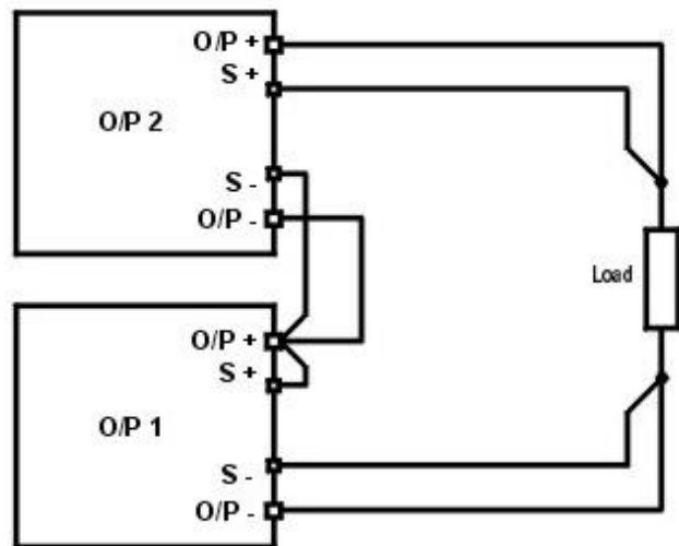
Series Wiring (Remote Sense) Serienschaltung (Remote Sense)
