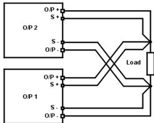
Parallel Wiring (Remote Sense) Parallelschaltung (Remote Sense)
