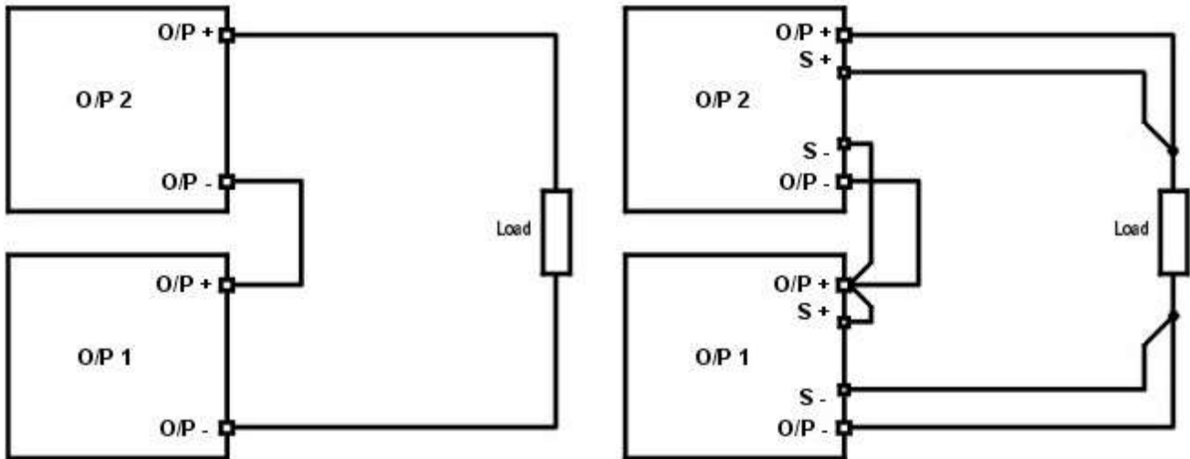
Series Wiring (Local Sense)
