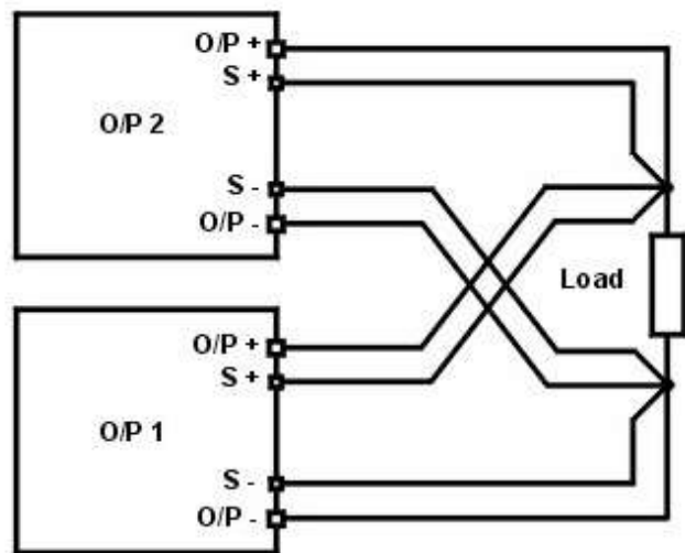
Parallel Wiring (Remote Sense) Parallelschaltung (Remote Sense)
