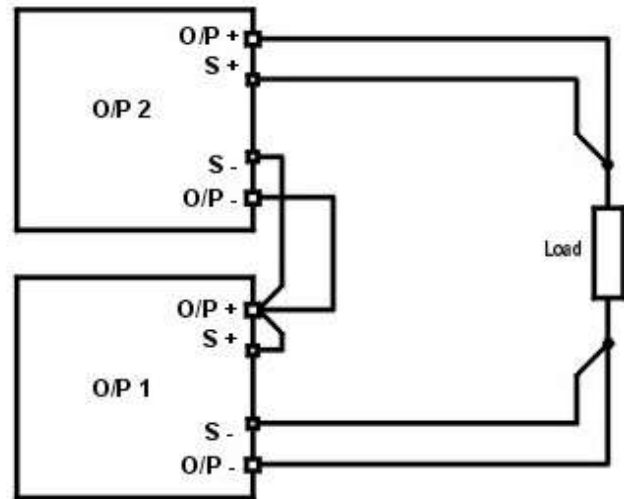
Series Wiring (Remote Sense) Serienschaltung (Remote Sense)
