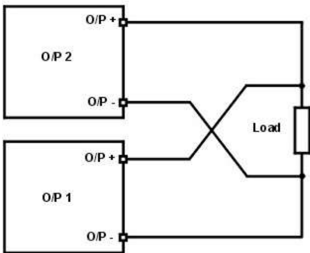
Parallel Wiring (Local Sense) Parallelschaltung (Local Sense)
