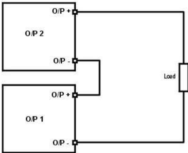
Series Wiring (Local Sense) Serienschaltung (Local Sense)
