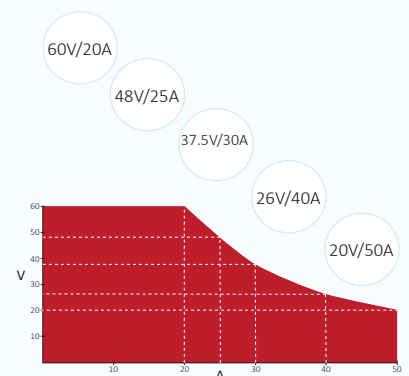
QPX1200S/SP PowerFlex
